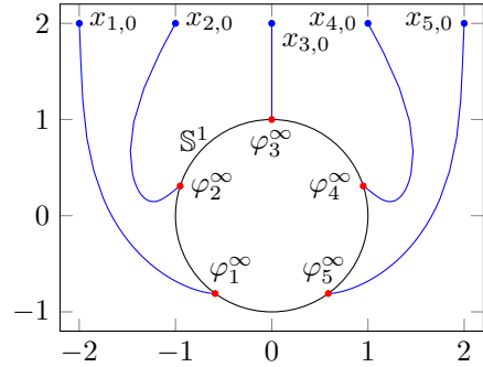
Fig. 3. Solution \varphi = (\varphi_1 \dots \varphi_5) (—) to the differential equation (15) together with its limiting value \varphi^\infty = (\varphi_1^\infty \dots \varphi_5^\infty) (●), which is contained in B from Fig. 2 for some initial condition x_0 = (x_{1,0} \dots x_{5,0}) (●), all on the example of the unit sphere M = \mathbb{S}^1 (○) and the cycle graph from Fig. 1
